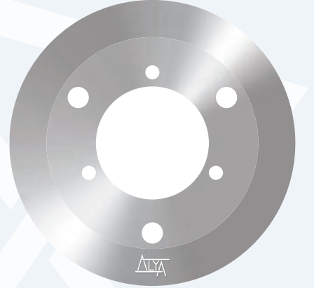
Dairesel Bıçak/Circular Knife 81.25x32x1mm, Çift Bileme/Double Bevel, 3x4.3mm Delik/Hole, 420 Paslanmaz/Stainless
